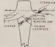
FIG. 219—When Blasting Tap Rooted Stumps, Charge May Be Loaded into a Hole Bored into the Tap Root at Angle Shown.
